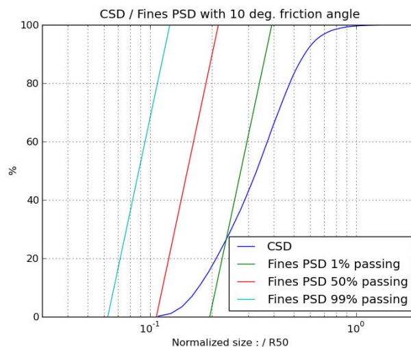
Figure 4: Particle Size Distribution (PSD) of fine particles associated to different passing percentage.
