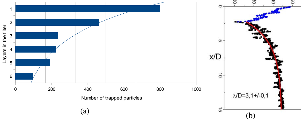
Figure 3: Vertical distribution of trapped particles in the filter; (a): DEM-PFV simulation, (b): experiment on glass beads, after [13].
