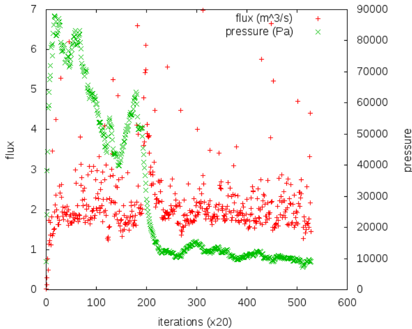
Figure 9: Flux and pressure values with an imposed flux value of 2 m³/s.
